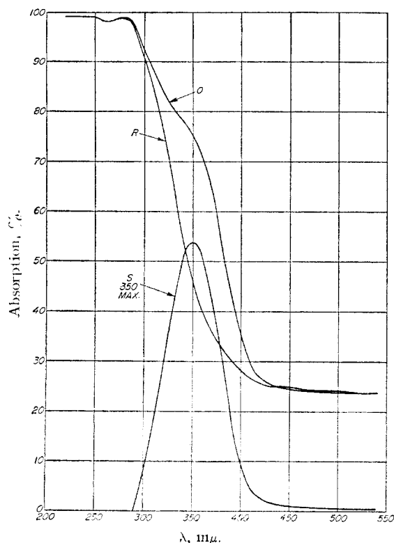
Fig. 5.—Absorption spectra: Q, spruce wood section mounted in nujol in comparison with a ground-surface quartz plate as reference; R, same except spruce section first bleached in buffered sodium peroxide; S, the unbleached section using the bleached section for reference, temperature -10^{\circ} .
